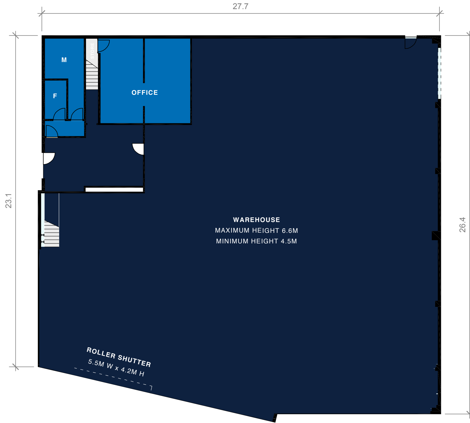
GROUND FLOOR
