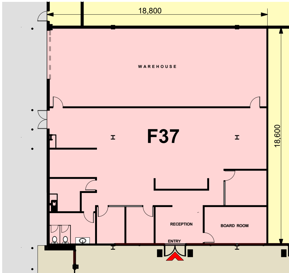
UNIT F37 FLOOR PLAN SCALE 1:200
